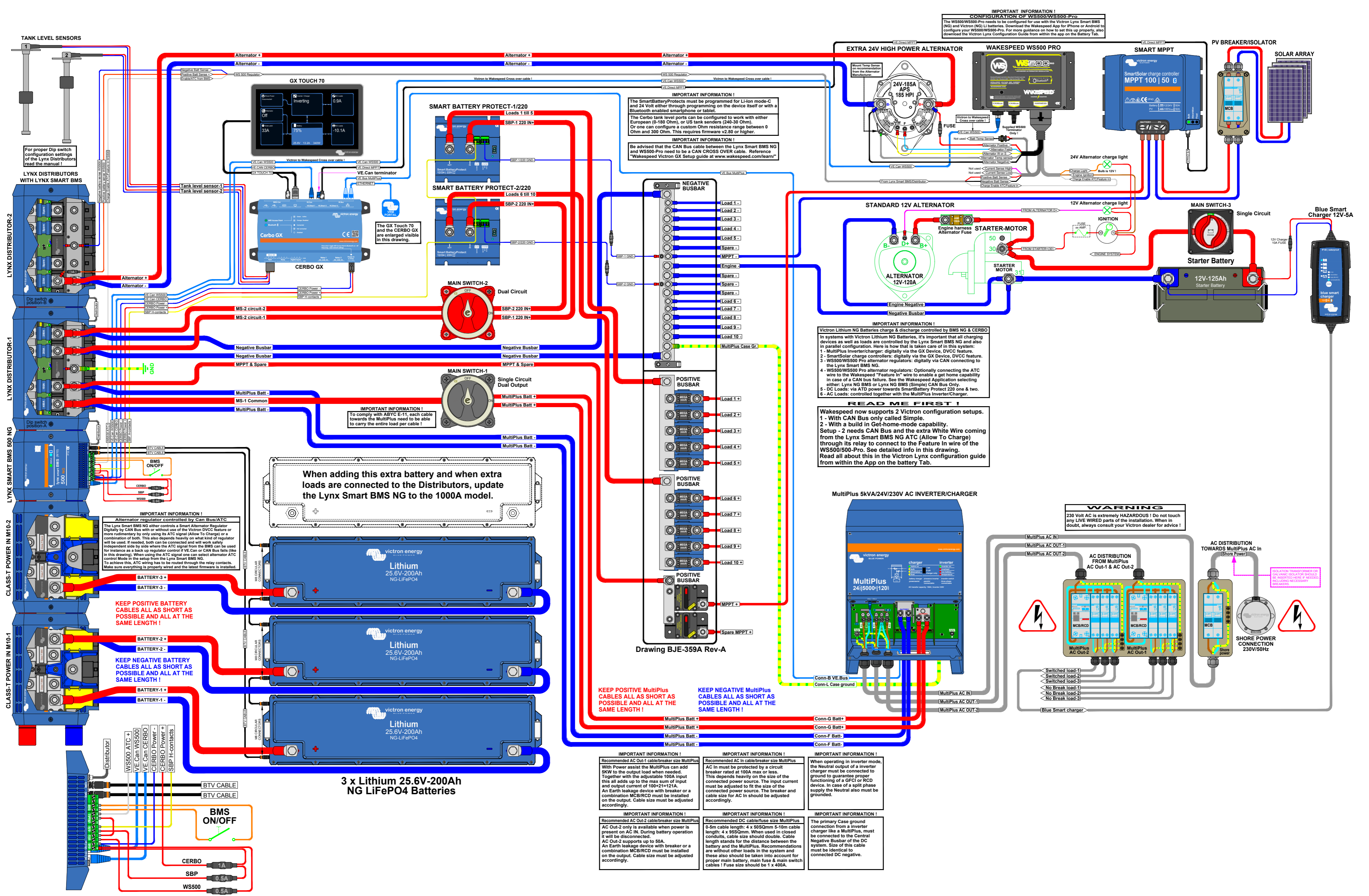
Lynx Smart BMS NG Enlarged connections
